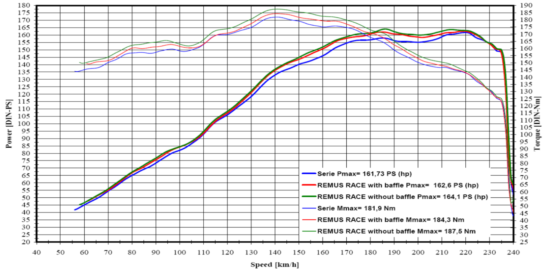
BMW K 1600 GT measured in Road mode
