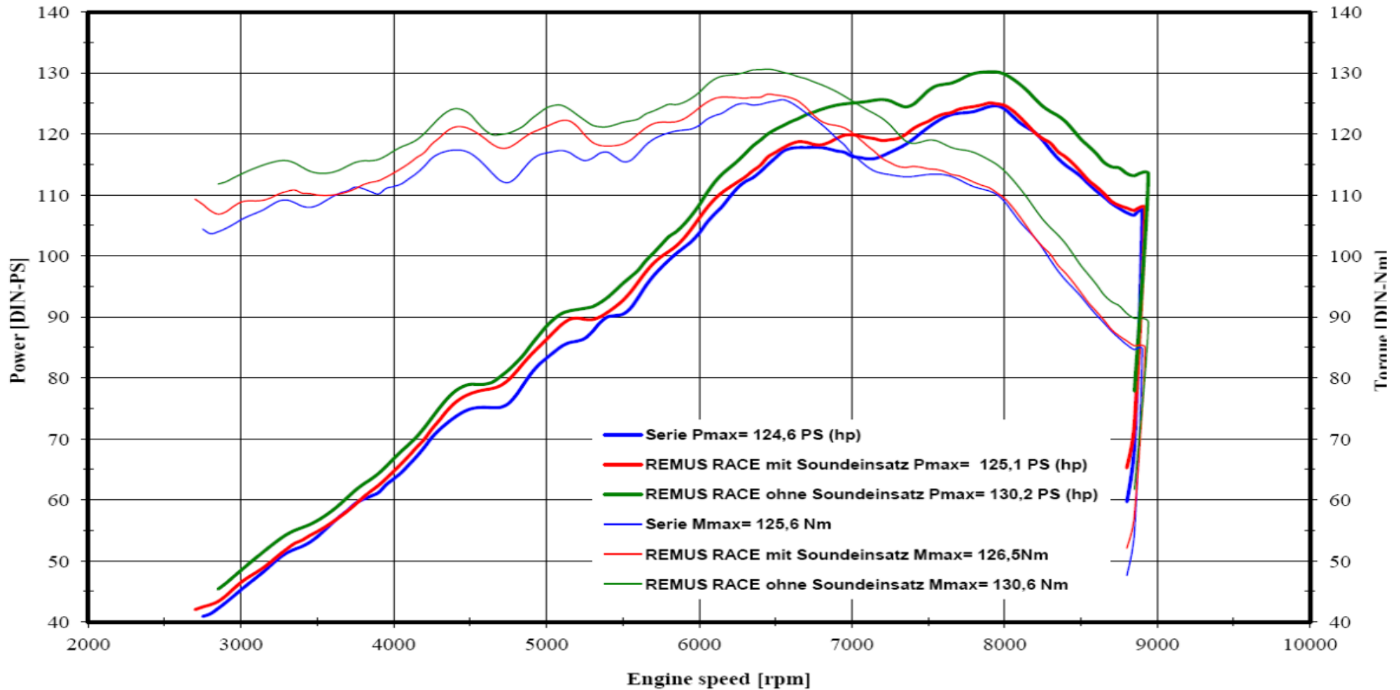
BMW R1200GS Complete Racing System
